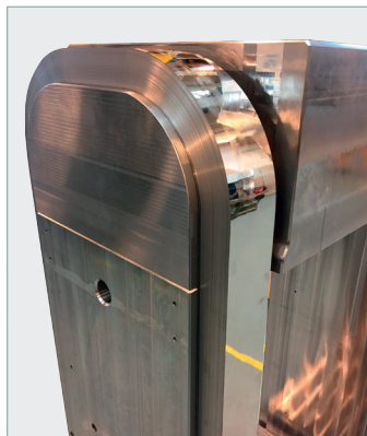
Stripwound press frame construction
